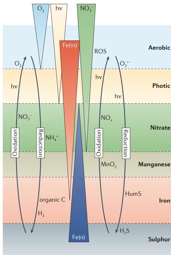
Figure 1 | Microbially and chemically mediated reactions that form the biogeochemical Fe cycle. Microbially mediated iron (Fe) redox reactions are shown on the left-hand side and abiotic Fe redox transformations are shown on the right-hand side, listed in a thermodynamic order (although some of these reactions may overlap in the natural environment). Within the oxic zone, microaerophilic Fe(II) oxidizers oxidize ferrous Fe (Fe(II)) using oxygen (O 2 ). Reactive oxygen species (ROS) can oxidize Fe(II), and superoxide (O 2 ·- ) can abiotically reduce ferric iron (Fe(III)). Within the photic zone, phototrophic microorganisms oxidize Fe(II) and photochemical reactions reduce Fe(III) that is bound to organic ligands (L). Mixotrophic and autotrophic nitrate (NO 3 - )-dependent Fe(II) oxidation is restricted to anoxic conditions in the denitrification zone. NO 3 - -reducing Fe(II)-oxidizing bacteria use Fe(II) as an electron donor. Fe-ammox bacteria couple the oxidation of ammonium (NH 4 + ) to Fe(III) reduction. Fe(II) can be chemically oxidized via chemodenitrification by reactive nitrogen (N) species. Fe(II) is abiotically oxidized by manganese (Mn) via surface-catalysed reactions. Fe(III)-reducing microorganisms can reduce Fe(III) coupled to the oxidation of various electron donors such as organic carbon (C) and H 2 . Electron-rich (that is, reduced) humic substances (HumS) abiotically reduce Fe(III) to Fe(II). Fe(III) is chemically reduced by hydrogen sulphide (H 2 S) to ferrous sulphide (FeS) species. The different gradients of O 2 , light, NO 3 - and Fe(II) and Fe(III) in a redox-stratified environmental system are shown, as well as where the different biotic and abiotic Fe redox transformations are expected to take place.
