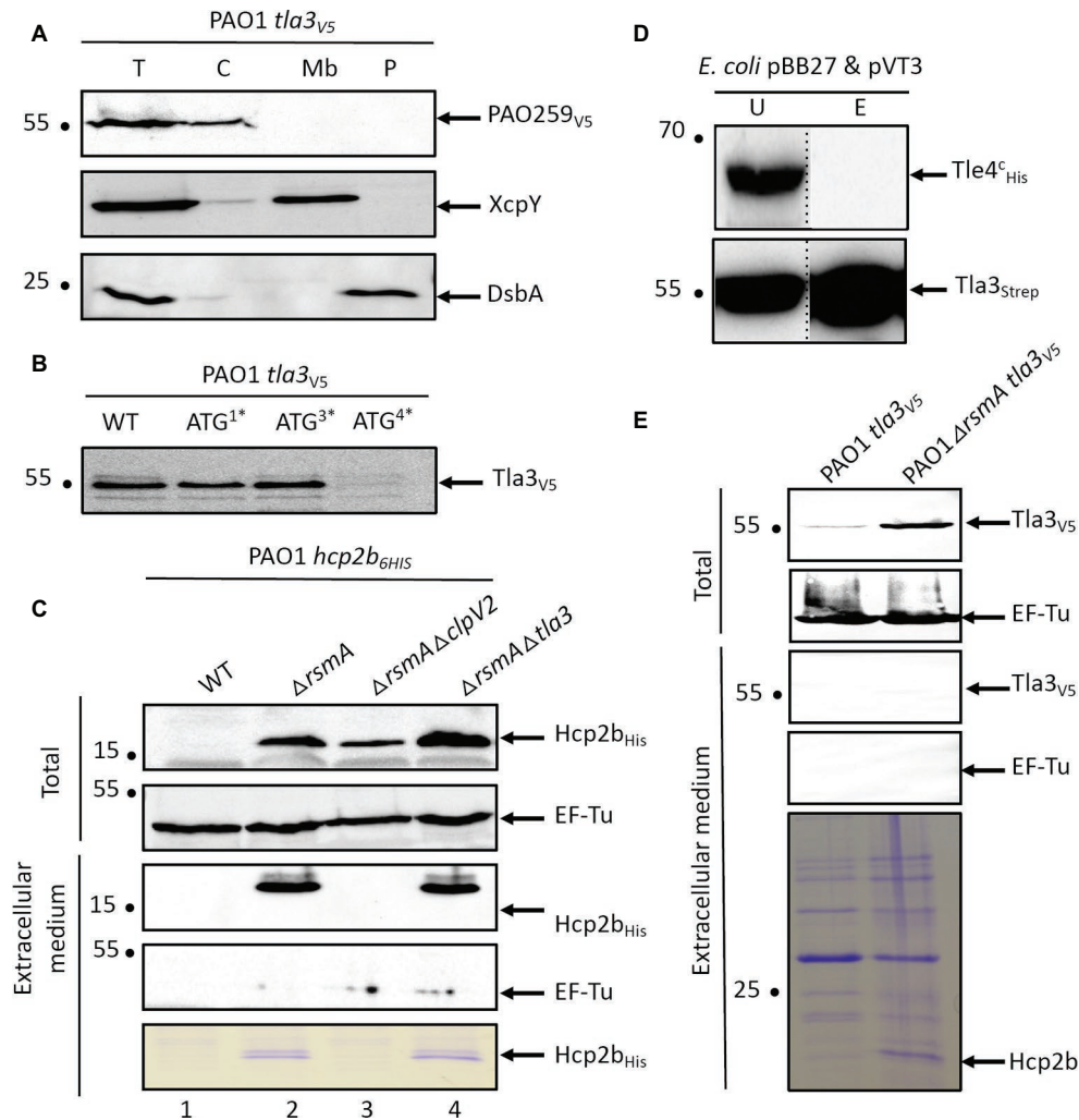
FIGURE 5 | (A) Tla3(PAO259) is a cytoplasmic protein of P. aeruginosa . Cells of P. aeruginosa PAO1 tla3 v5 were subjected to fractionation and immunoblotting using antibodies directed against the V5 tag, XcpY and DsbA. XcpY and DsbA were used as membrane and periplasmic controls, respectively. T, whole cell; C, cytoplasm; Mb, total membrane; P, periplasm. (B) The annotated ATG drives the initiation of translation of tla3 in P. aeruginosa . Immunodetection of Tla3 v5 with anti-V5 antibodies produced in a WT background or in strains in which one of the four predicted ATG in tla3 have been substituted in ATA. The number followed by a star indicates which ATG from Supplementary Figure S1 ATG i corresponds to the annotated ATG. (C) Tla3 is not required for Hcp2b secretion. Immunodetection of Hcp2b His with anti-His antibodies produced in a WT background (line 1) or in strains deleted for rsmA (lines 2–4) and clpV2 (line 3) or tla3 (line 4). The strains were grown at 25°C for 24 h and total bacteria were separated from extracellular medium. Anti-EF-Tu is used as a lysis control. The extracellular medium proteins were also stained with Coomassie-blue. (D) Tla3 does not interact with Tle4. Copurification assay on StrepTactin column of Tla3 c STREP with Tle4 His produced in E. coli BL21(DE3)pLysS from pBB27 and pVT3 respectively. Legend is as in Figure 4 . (E) Tla3 is not secreted. Immunodetection of Tla3 v5 with anti-HV5 antibodies produced in a WT background (line 1) or in strain deleted for rsmA (line 2). The strains were grown at 25°C for 24 h and total bacteria were separated from extracellular medium. Anti-EF-Tu is used as a lysis control. The extracellular medium proteins were also stained with Coomassie-blue. (A–E) The position of the proteins and the molecular mass markers (in kDa) are indicated.
